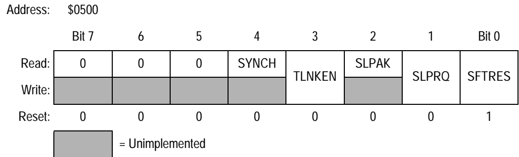
Figure 21-15. Module Control Register 0 (CMCR0)
