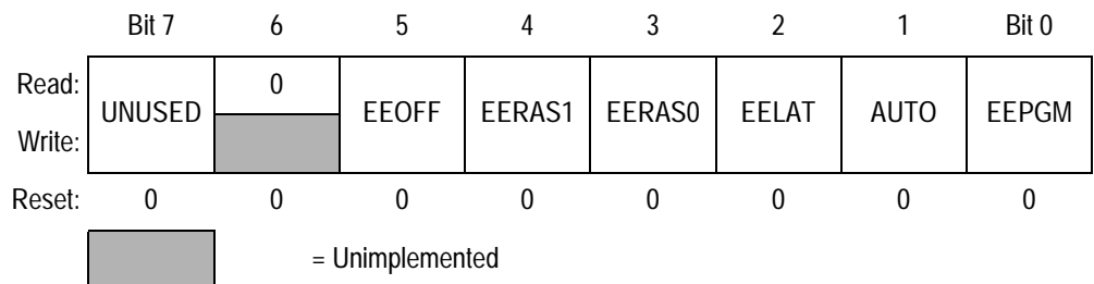
Figure 6-2. EEPROM-2 Control Register (EE2CR)
