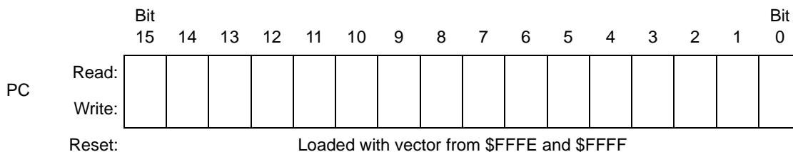
Figure 7-5. Program Counter (PC)
