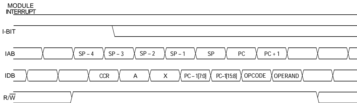
Figure 8-8. Interrupt Recovery
