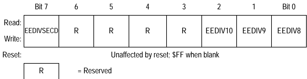
Figure 5-7. EEPROM-1 Divider Non-Volatile Register High (EE1DIVHNVR)
