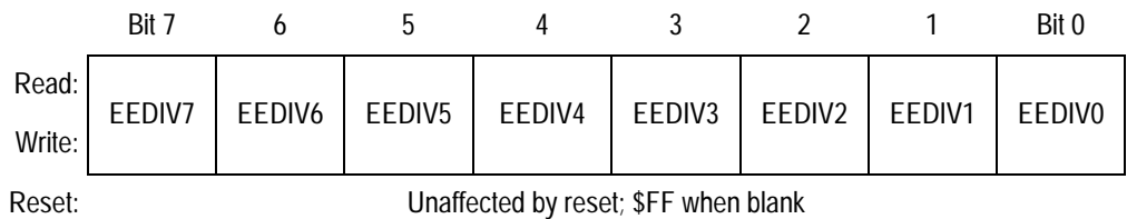
Figure 5-8. EEPROM-1 Divider Non-Volatile Register Low (EE1DIVLNVR)
