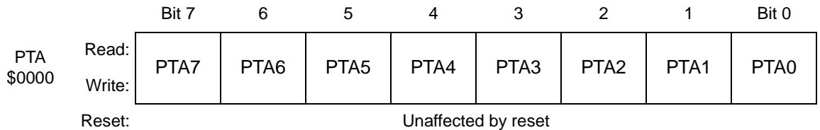
Figure 20-1. Port A data register (PTA)
