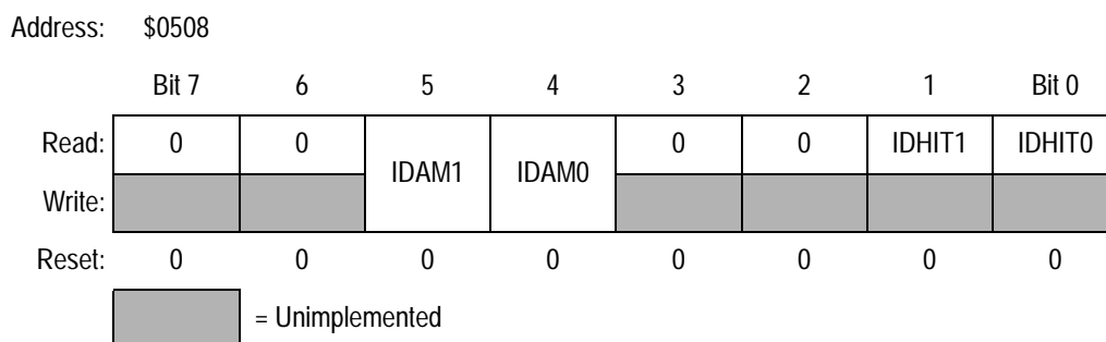
Figure 21-23. Identifier Acceptance Control Register (CIDAC)
