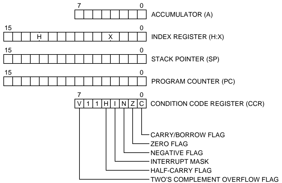
Figure 7-1. CPU Registers
