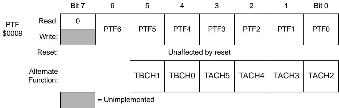
Figure 20-16. Port F Data Register (PTF)
